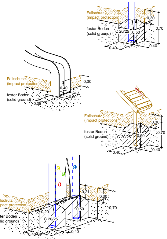
Alternativ: Fundament flach/kantig (Alternative: Foundations plain/edged)
