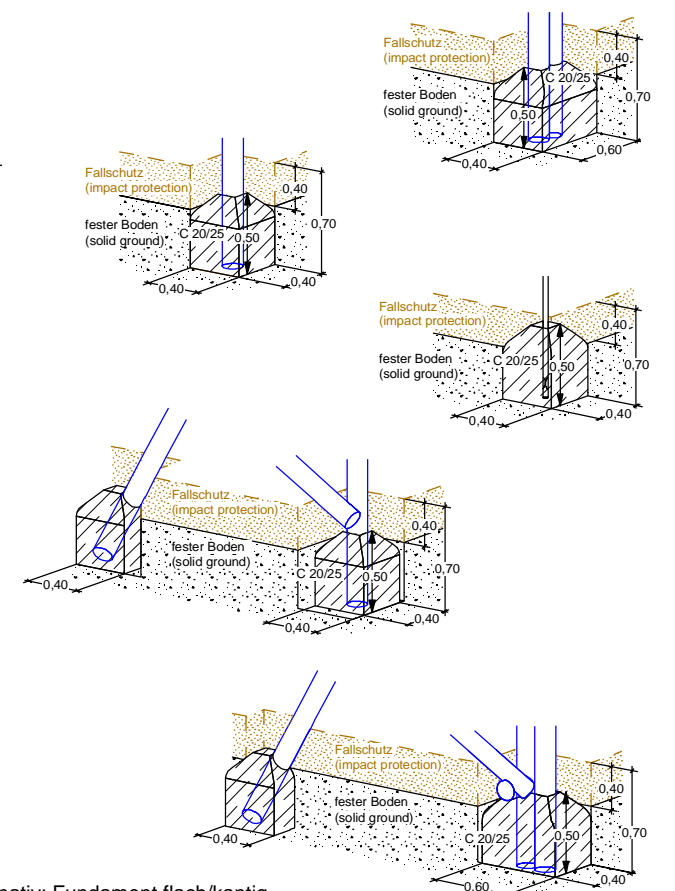
Alternativ: Fundament flach/kantig (Alternative: Foundations plain/edged)
