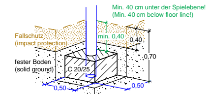
Alternative Grundfläche 12.5% (1/8) größer. In this version base area 12.5% (1/8) larger.
