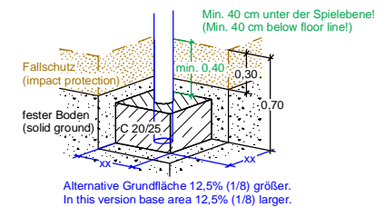
Alternativ: Fundament flach/kantig (Alternative: Foundations plain/edged)
