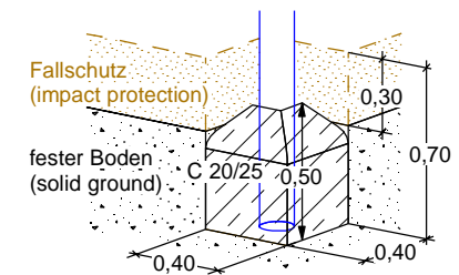
Alternativ: Fundament flach/kantig (Alternative: Foundations plain/edged)
